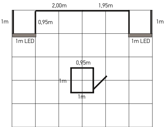
top view height 3m
