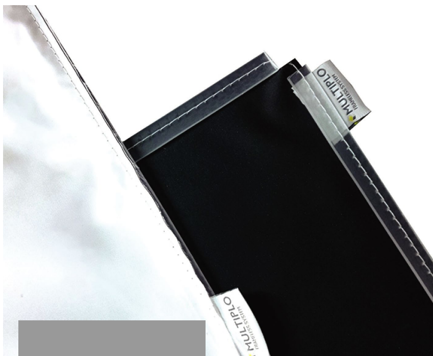
Material: 100% Polyester Weight: 195 gr/m 2 Thickness: 250 µm Elasticity: ca. 1% Transmission factor: 38%
