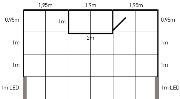
top view height 3m
